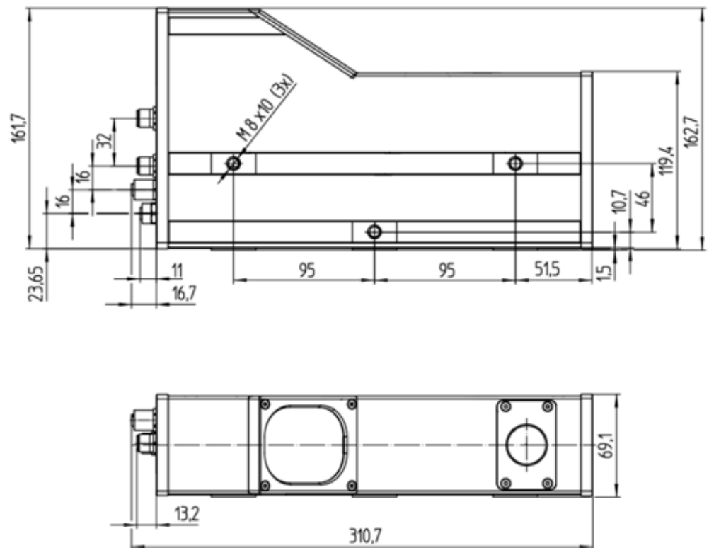
Figure 4.2- Camera IVC-3D 50 (not to scale). The mounting holes have the same position on back and upper side.
