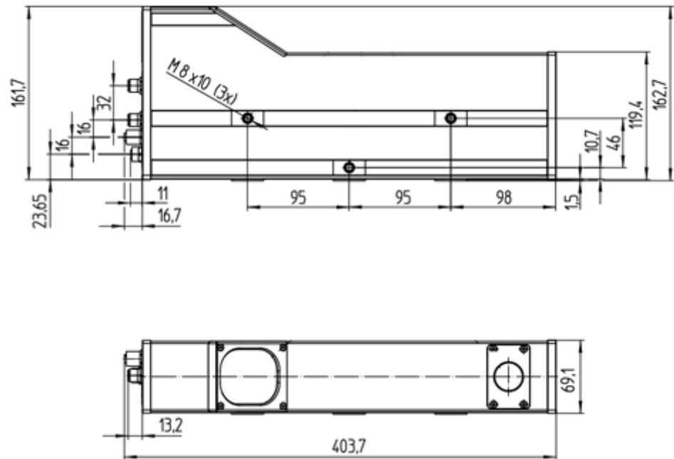
Figure 4.1- Camera IVC-3D 200 (not to scale). The mounting holes have the same position on back and upper side.
